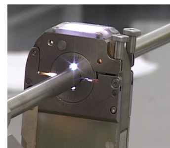
Orbital welding (TIG welding - mainly used in pharma and food indus- try)
